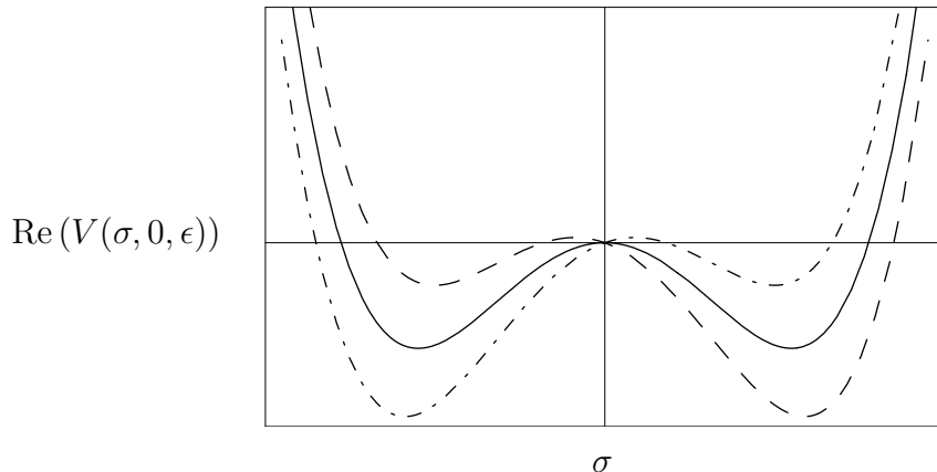
Figure 2: Projection of the real part of the meson potential depending on \sigma . The sign of the explicit symmetry breaking term induces the choice of the global minimum and hence the vacuum expectation value. The solid curve is the potential without explicit symmetry breaking. The dashed and dashed dotted curves result from x = +\epsilon and x = -\epsilon respectively.
